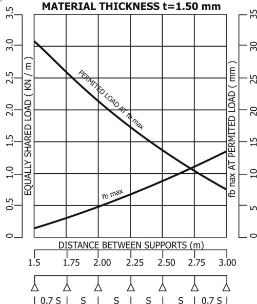
CABLE TRAY H:110 LOADING DIAGRAM MATERIAL THICKNESS t=1.50 mm
